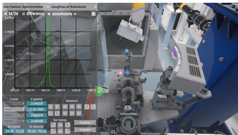
Figure 3: The Von Hamos spectrometer in operating position. with the read-out of the Jungfrau detector as well as the settings for the position to the left.
