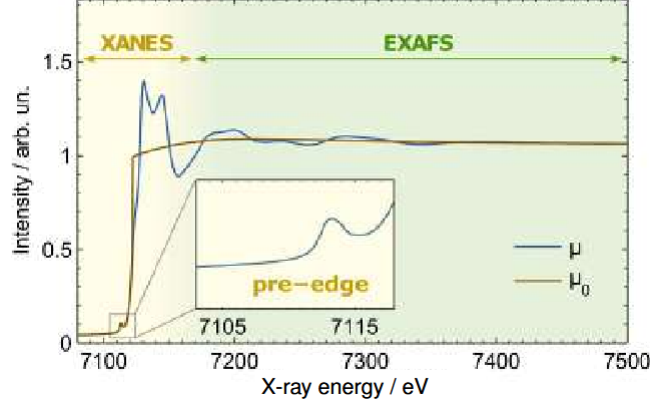
Figure 1: X-Ray absorption spectrum of [\text{Fe}(\text{terpy})_2]^{2+} (terpy: terpyridin) at the Fe K edge displaying the XANES and EXAFS regions including the background absorption contributions \mu_0 . The inset zooms into the weak pre edge features [4].
